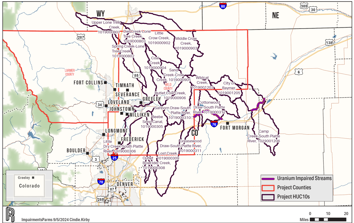
Figure B-7. Uranium Impairments.
