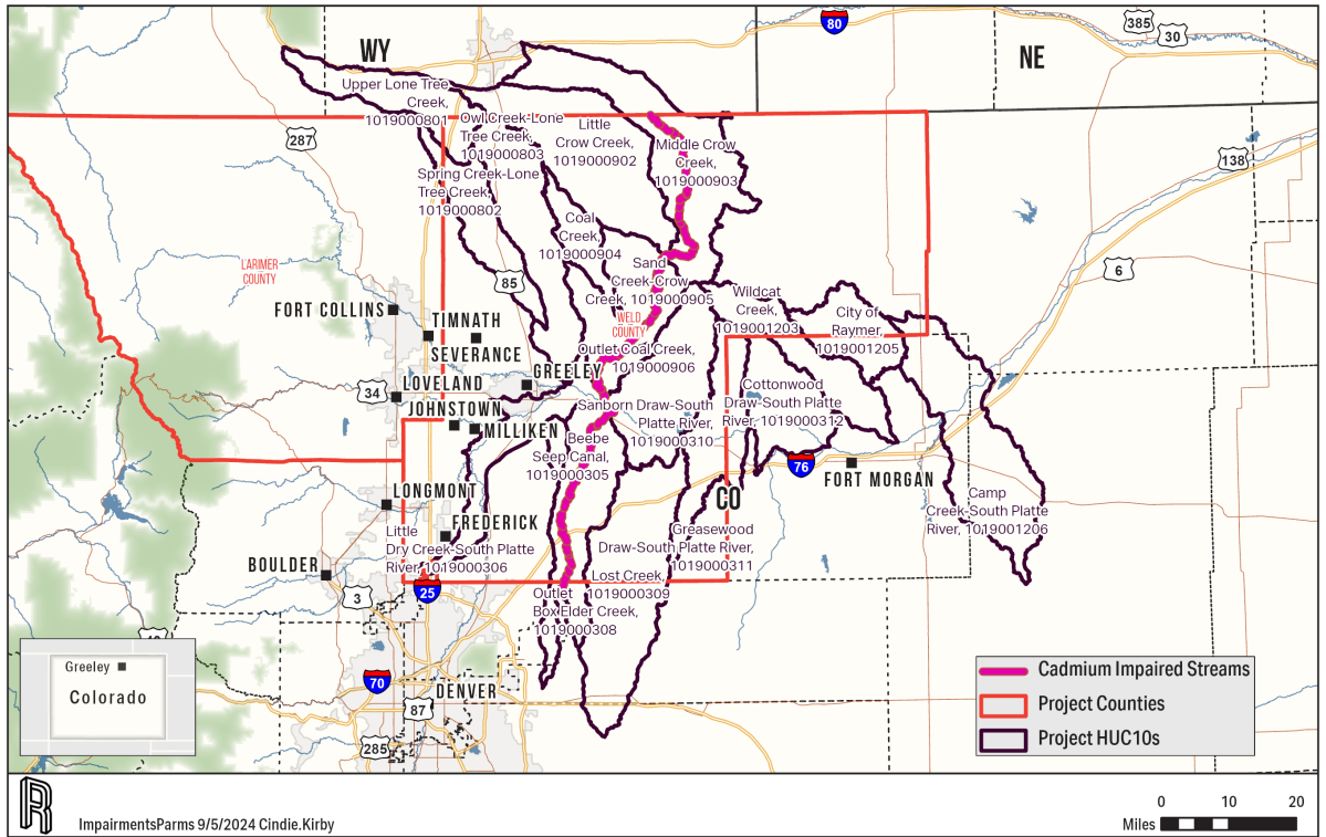
Figure B-5. Cadmium Impairments.
